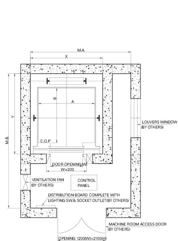
PLAN OF HOISTWAY & MACHINE ROOM
