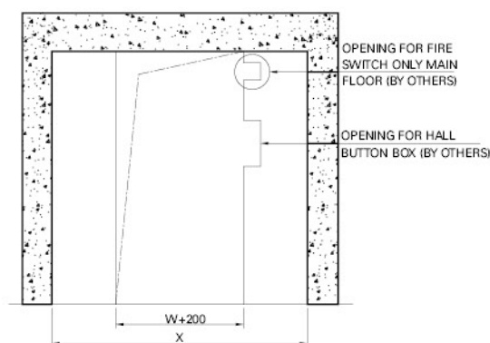
FRONT VIEW OF ENTRANCE
